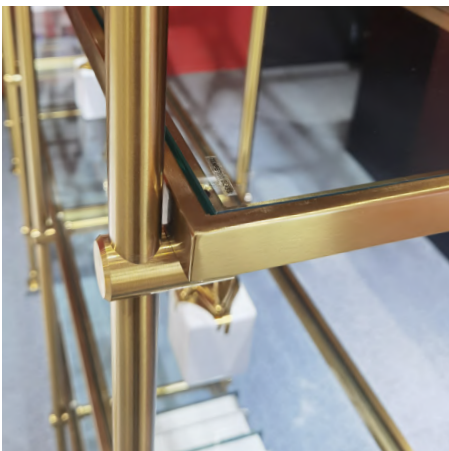
STAINLESS STEEL AND GLASS SHELF SUPPORT
